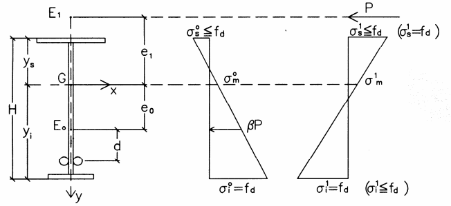
Figure 7. Limit points.
