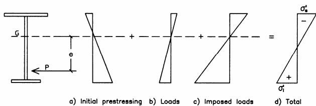
Figure 4. Condition at service.
