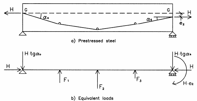
Figure 11. Equivalent loads.
