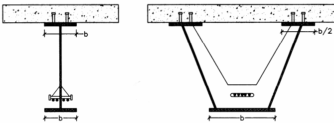
Figure13. Typical sections.
