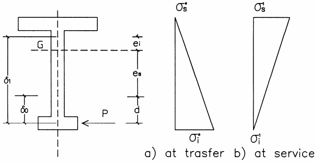
Figure 6. Prestressed concrete girder.
