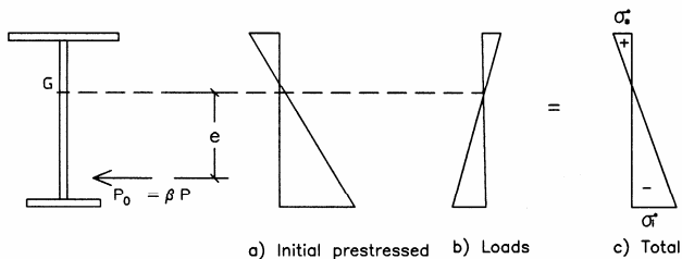
Figure 3. Condition at transfer.
