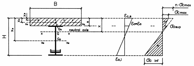
Figure 14. Prestressed composite girder.
