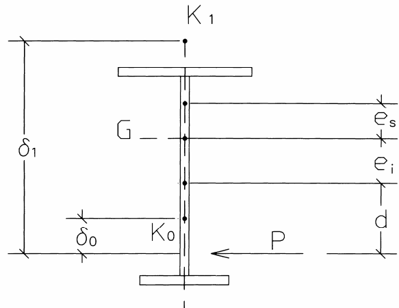
Figure 5. Representations of kern points e_i and e_s
